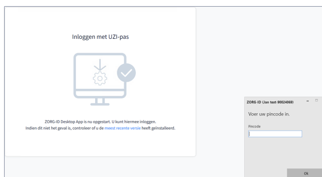
Figure 26: Invoer pincode
