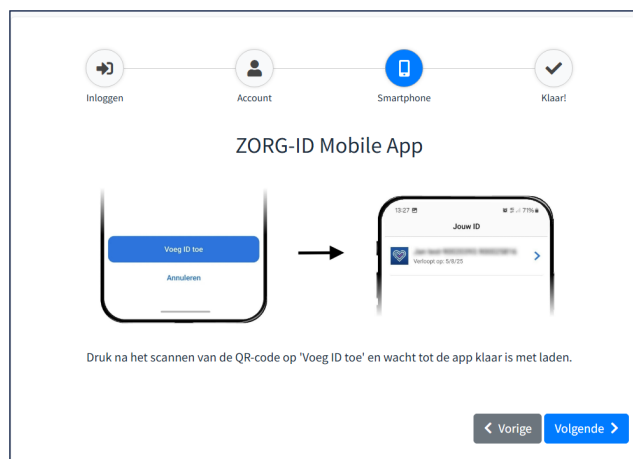
Figure 17: ID registratie
